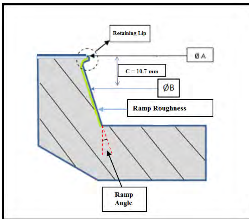
Figure 1. Duo Cone Seal Dimensions and Measures
